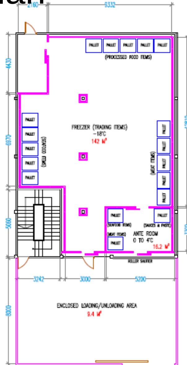
1ST STOREY UNIT LAYOUT TOTAL AREA SIZE @ 308 \text{ M}^2
